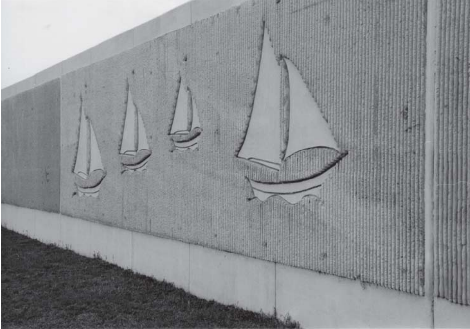
Figure 11-3. Use of fractured ribs highlights artistic design
