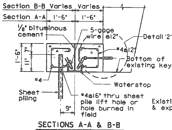
Figure 7-11. Permanent water stop repair measures (Continued)
