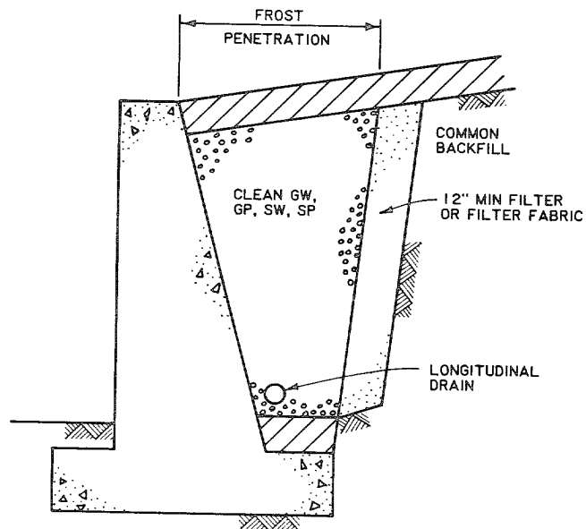
Figure 6-5. Drainage system to prevent frost penetration behind retaining wall (after Department of the Navy 1982a)
