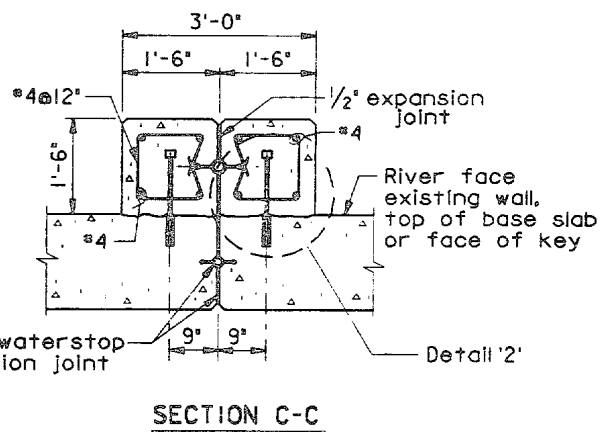
Figure 7-11. Permanent water stop repair measures (Continued)
