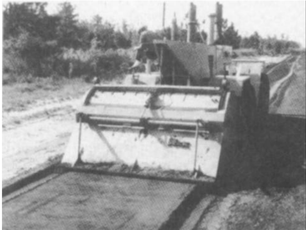
Figure 4-49. Single-shaft rotary mixer without asphalt.
