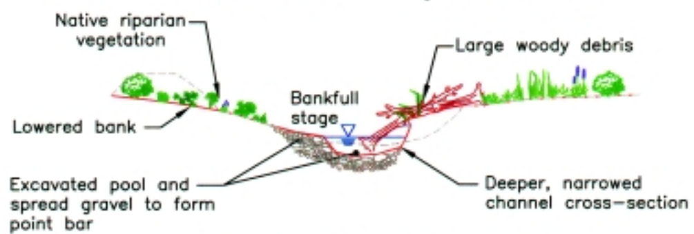
SECTION A - A' - Enhanced Condition
