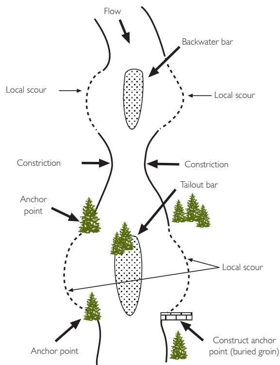
Figure 2-8. Tailout and backwater bars.
