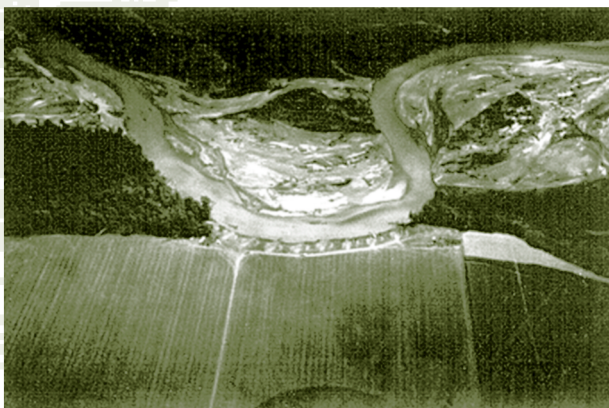
Figure 5-4. Plan view of erosion on the Nooksack River.
