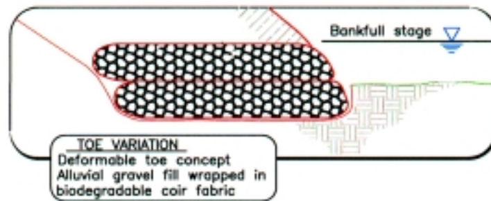
DEFORMABLE TOE
