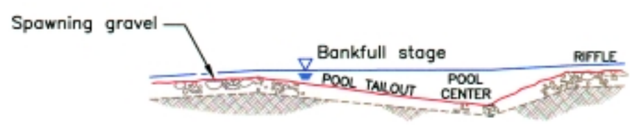
SECTION B - B' - Enhanced Condition
