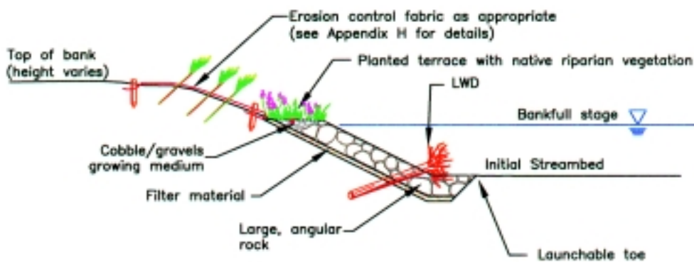
RIPRAP TERRACED WITH ROUGHENED ROCK TOE, LWD, RIPARIAN PLANTINGS, AND FABRIC COVERED UPPER BANK
