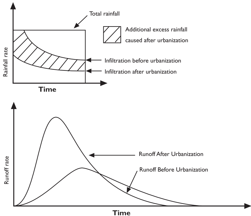
Figure D-5. Urban Hydrograph 2
