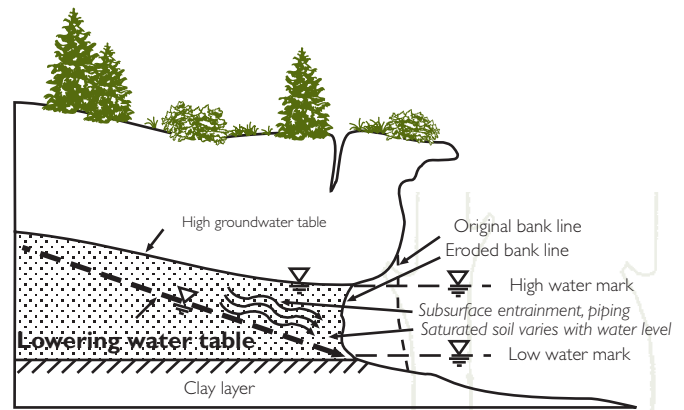
Figure 2-14. Subsurface entrainment, or piping.
