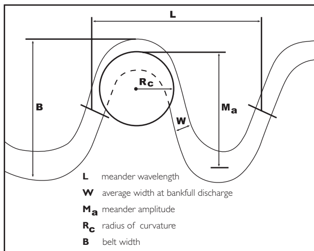
Figure 3-5. Channel planform characteristics.
