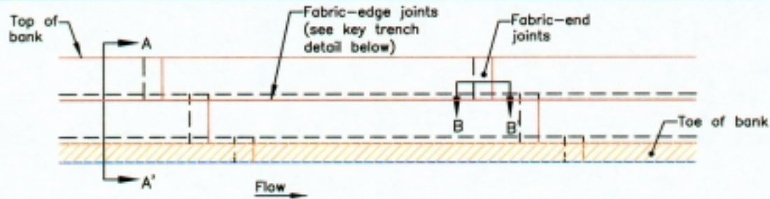
PLAN VIEW OF FABRIC-COVERED BANK SHOWING FABRIC ROLLS ORIENTED PARALLEL TO FLOW
