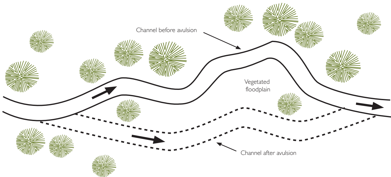
Figure 3-17. Avulsion.
