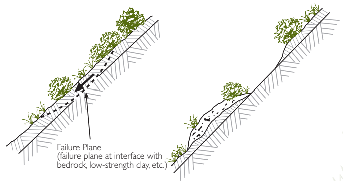
Figure 2-16. Translational slide.
