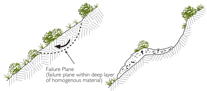
Figure 2-15. Rotational slide.
