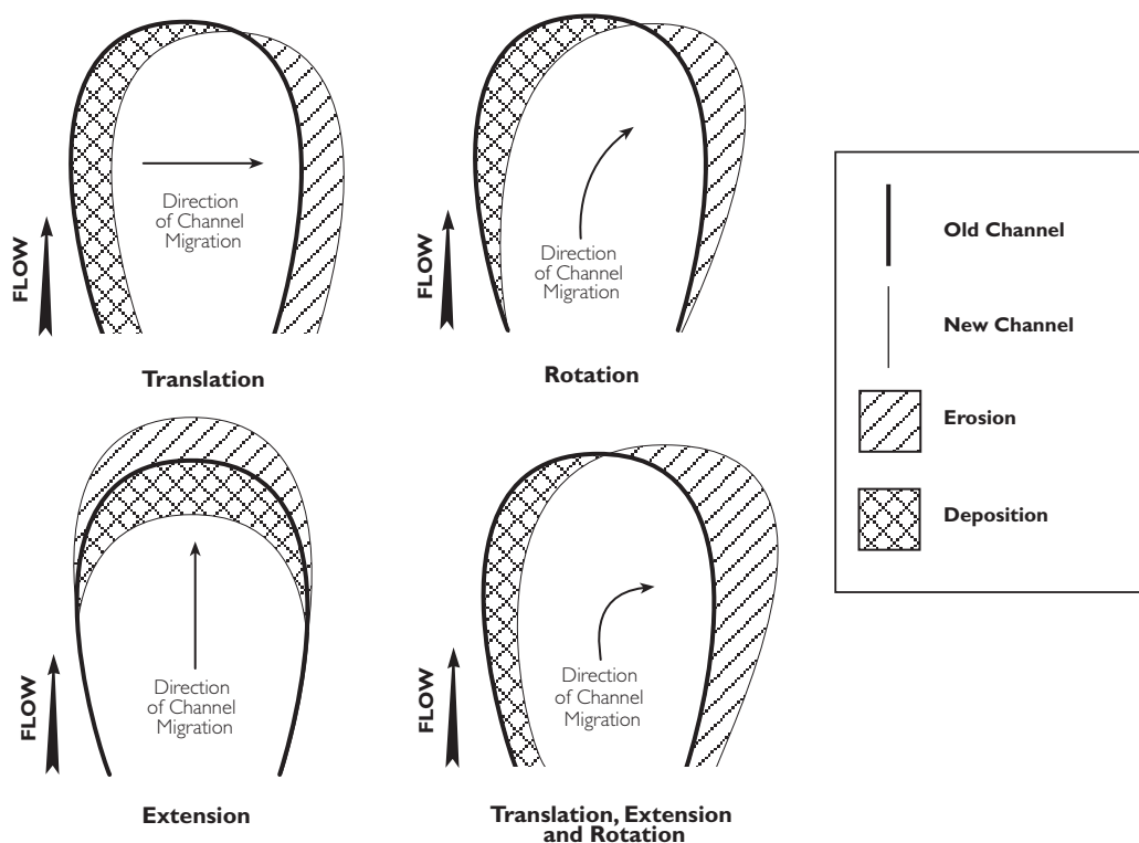
Figure 3-8. Migration patterns.
