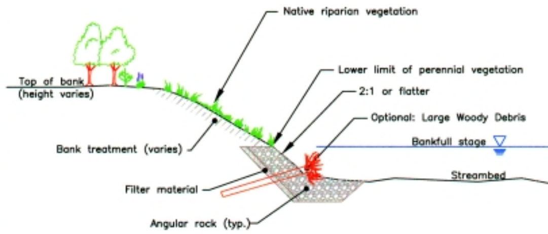
LAUNCHABLE TOE
