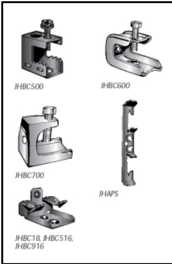
Beam Clamps
