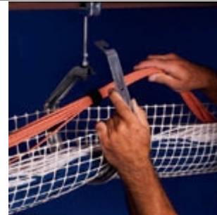
3. Place cable in mesh. Secure with steel retaining strap. (The removable retaining strap allows for future cables.)
