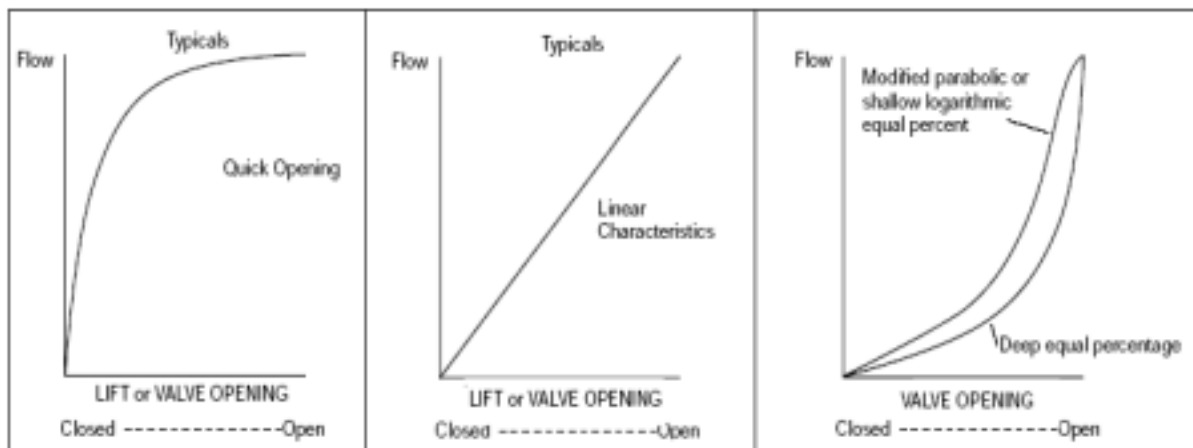
Response curve of various valves
