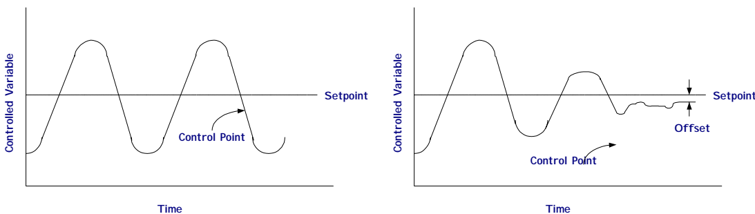
UNSTABLE SYSTEM UNDER PROPORTIONAL CONTROL
