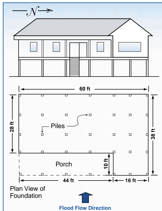
Figure 11-15 Building elevation and plan view of pile foundation.
