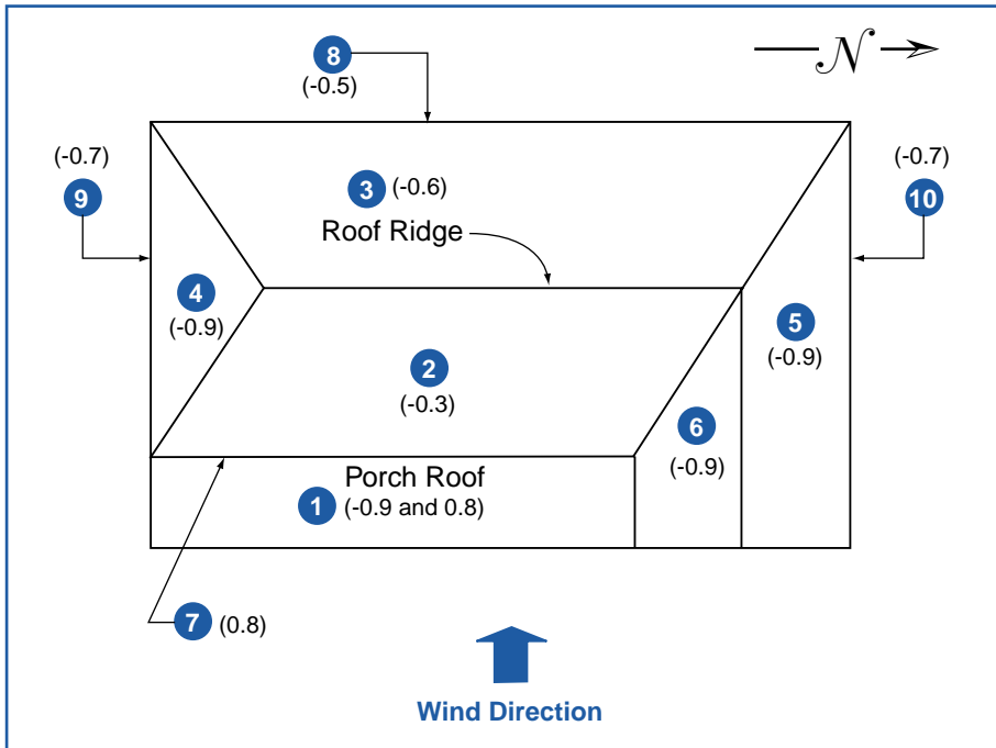
Figure 11-23 Wind pressure zones for MWFRS. The external pressure coefficients ( C_p ) for the 10 zones indicated are provided here for the case of wind direction from the east.
