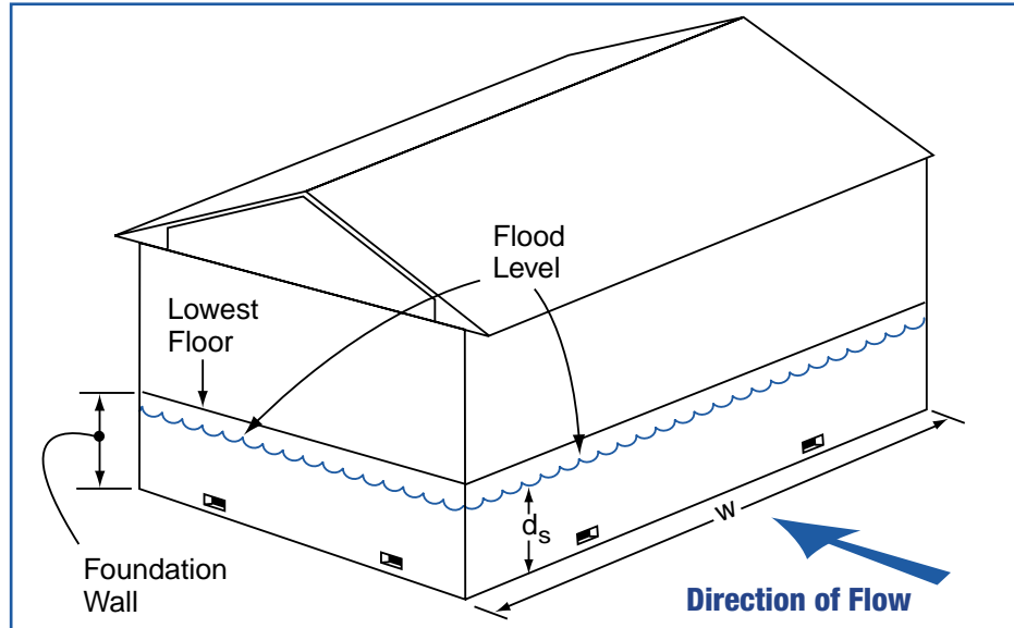
Figure 11-10 Determining drag coefficient from width-to-depth ratio. Note that the lowest floor of the building shown here is above the flood level.
