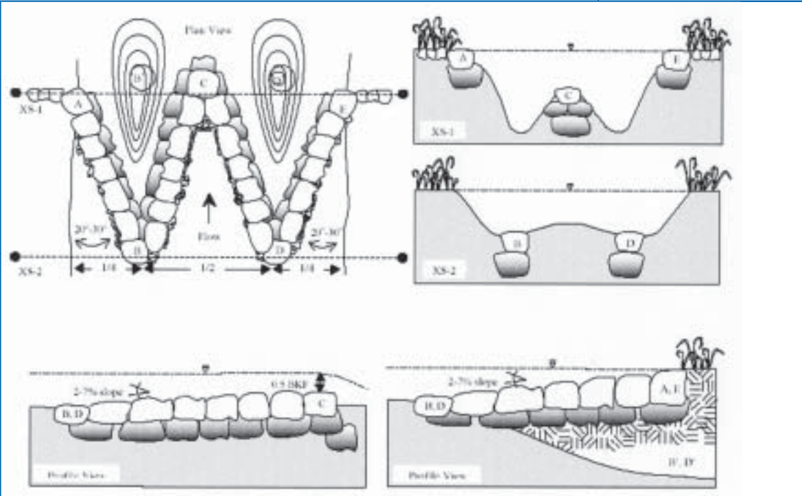
Figure 8.12 Plan, cross section and profile views of the W-weir Rosgen 2001c
