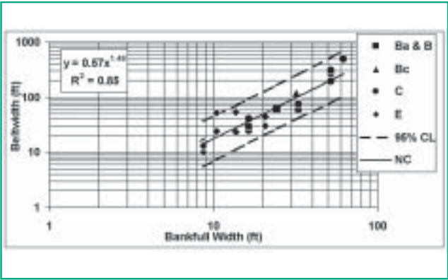
Figure 6.5 Belt width as a function of bankfull width Clinton et al., 1999
