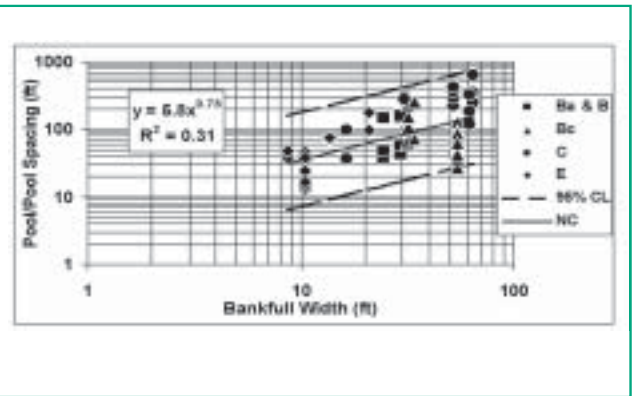
Figure 6.8 Pool-to-pool spacing as a function of bankfull width Clinton et al., 1999
