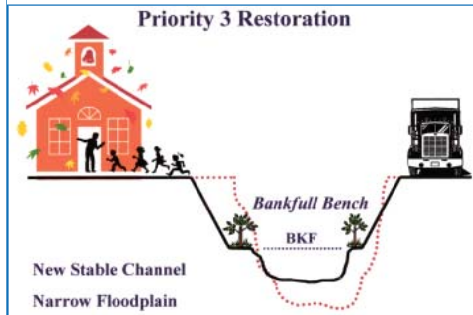
Figure 5.4 Cross section of a Priority 3 restoration project
