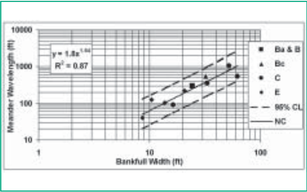
Figure 6.7 Meander wavelength as a function of bankfull width Clinton et al., 1999
