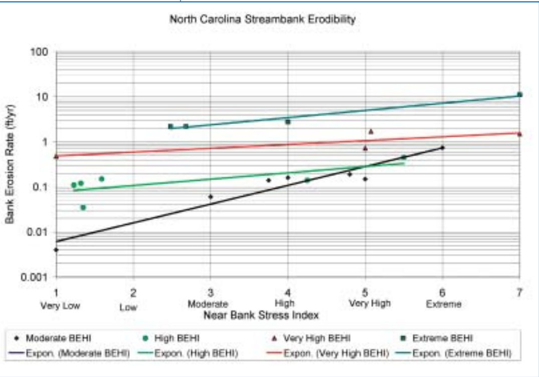
Figure 3.13 Measured streambank erosion rates in relation to near-bank stress and BEHI score Source: Natural Resource Conservation Service, NC State University and NC Division of Soil and Water Conservation.
