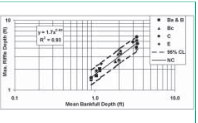
Figure 6.10 Max riffle depth as a function of mean bankfull depth Clinton et al., 1999
