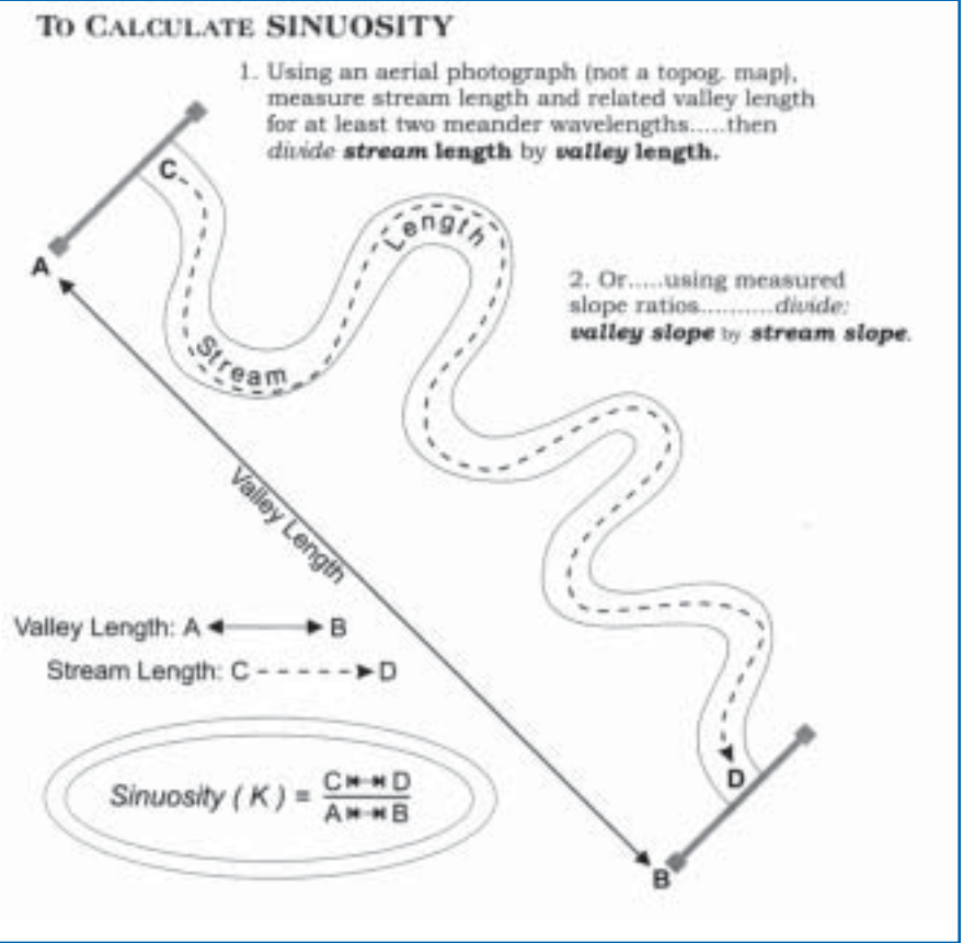
Fig. 2.6 Sinuosity measurement Rosgen, 1998b, 211
