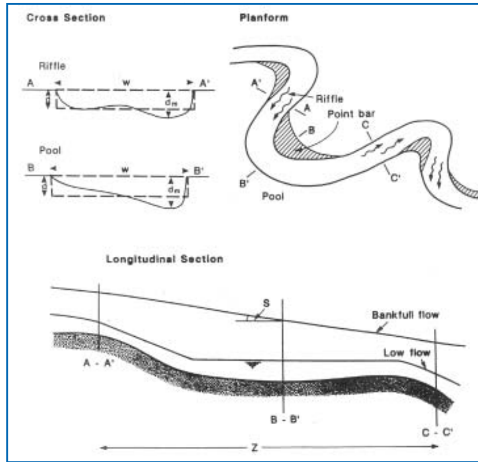
Figure 1.7 Features of natural streams From Hey, R.D. and Heritage, G.L. (1993). Draft guidelines for the design and restoration of flood alleviation schemes. National Rivers Authority, Bristol, UK, R&D Note 154
