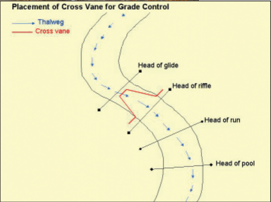
Figure 8.8 Cross vane showing placement and measurements * The lowest slope is most desirable, but in small streams a narrow channel may necessitate higher slopes (10 to 20 percent).
