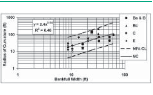
Figure 6.6 Radius of curvature as a function of bankfull width Clinton et al., 1999
