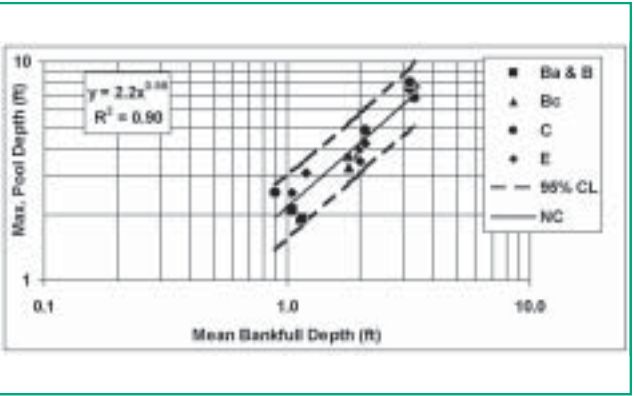
Figure 6.9 Max pool depth as a function of riffle mean bankfull depth Clinton et al., 1999
