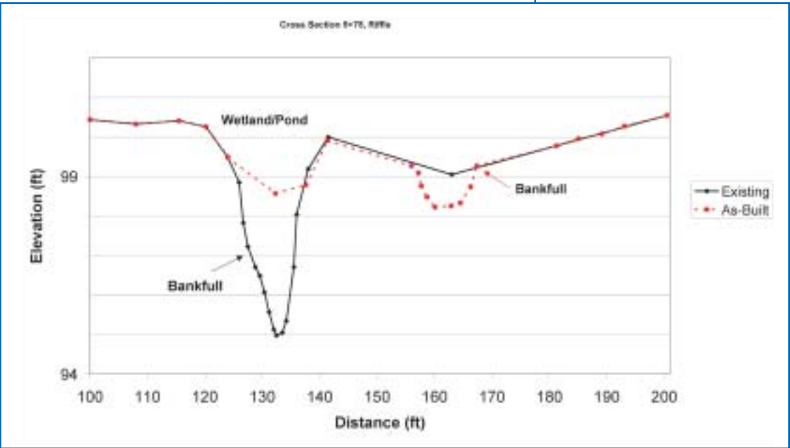
Figure 5.5 Cross-section survey of Yates Mill Pond tributary-restoration project
