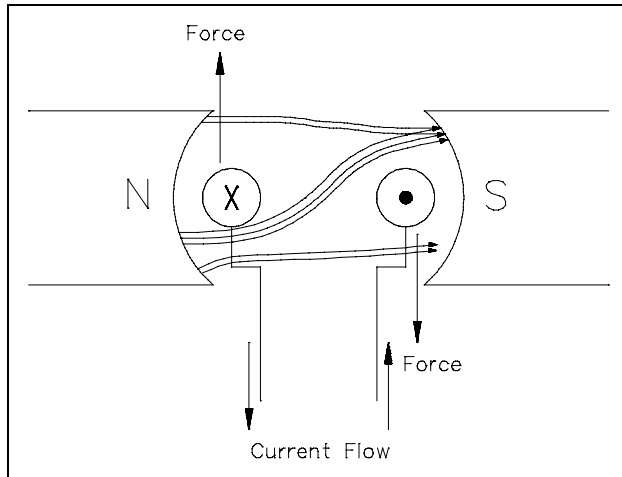
Figure 3 Motor Action
