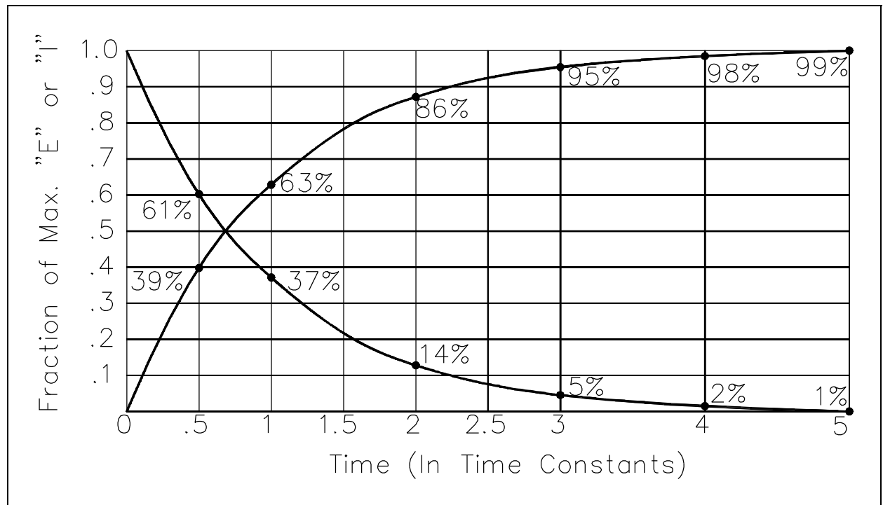
Figure 7 Time Constant
