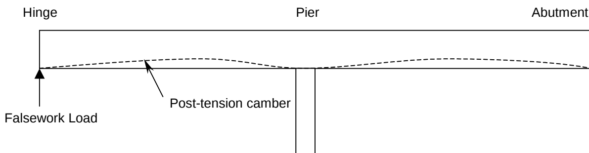
CAMBER DIAGRAM
