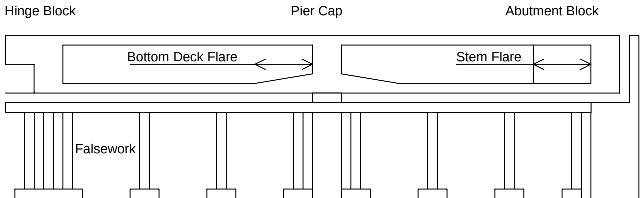
TYPICAL LONGITUDNAL SECTION
