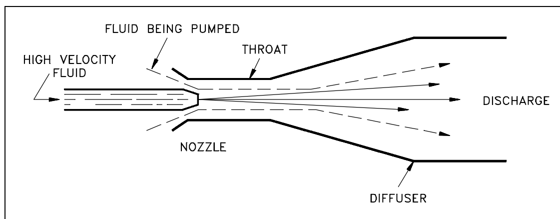
Figure 10 Jet Pump
