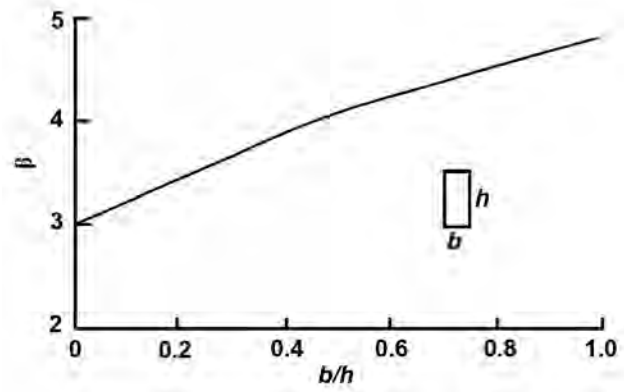
Figure 9-6. Coefficient \beta for computing maximum shear stress in torsion of rectangular member (Eq. (9-24)).
