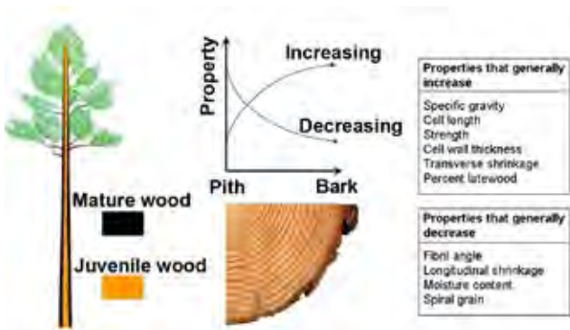
Figure 5–9. Properties of juvenile wood.
